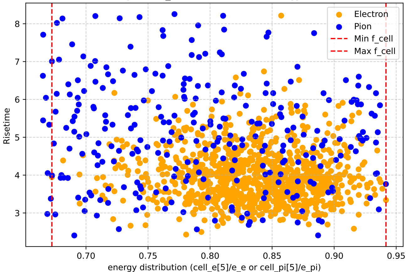
Scatter plot of f_cell vs risetime for energy 1.0GeV
